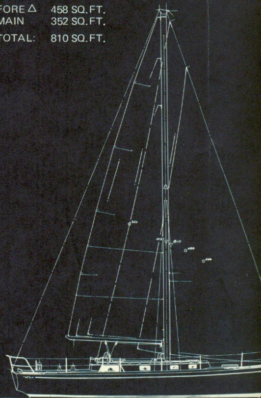
L.O.A. 40'9" D.W.L. 32'6" BEAM 12'6" DRAFT 6'0"
