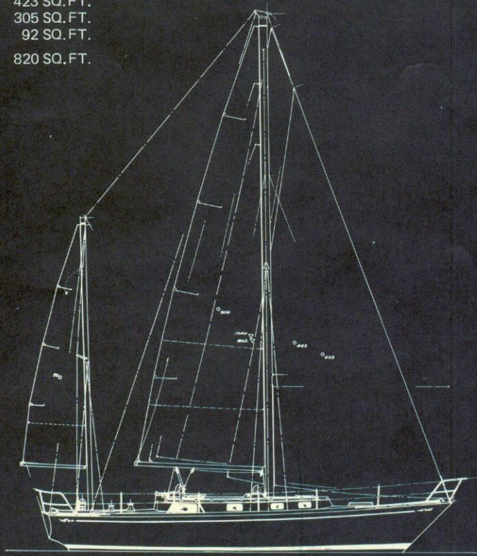
L.O.A. 40'9" D.W.L. 32'6" BEAM 12'6" DRAFT 6'0"
